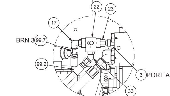
DETAIL 2E2 LEFT TURN SHUTTLE SOME PARTS REMOVED FOR CLARITY
